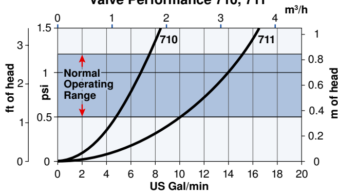
Valve Performance 710, 711
