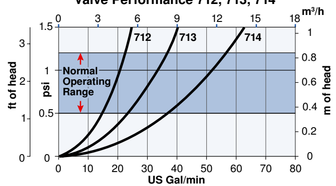
Valve Performance 712, 713, 714
