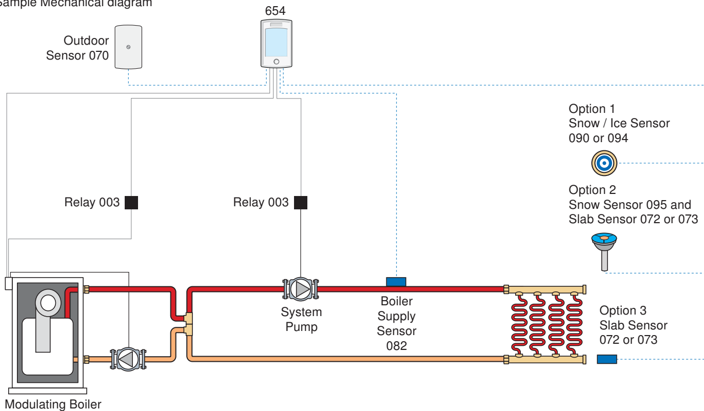
Sample Mechanical diagram
