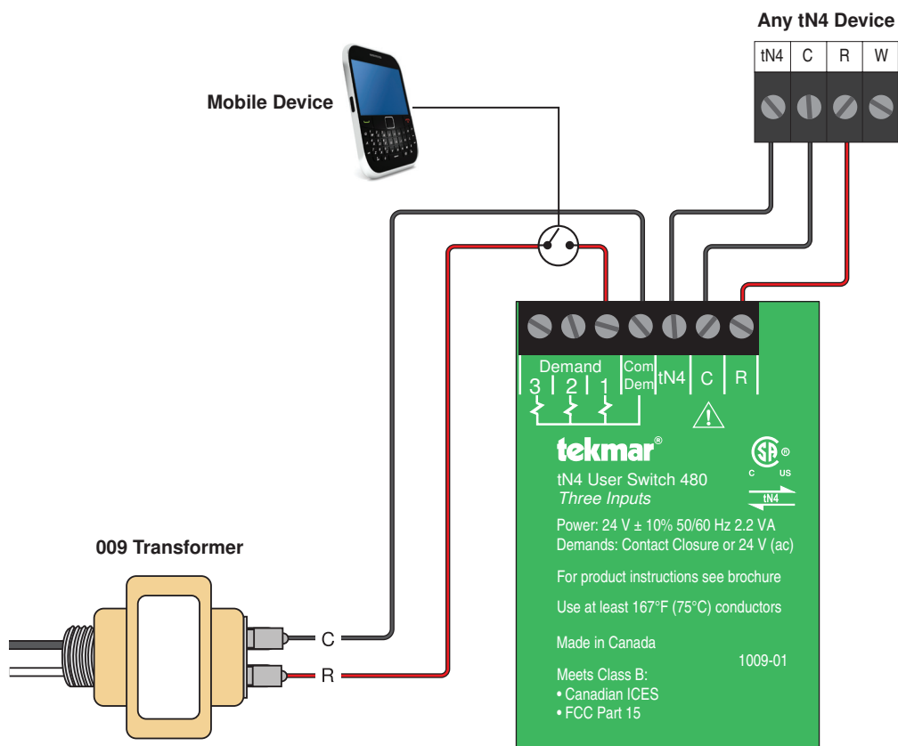
Sample Electrical diagram
