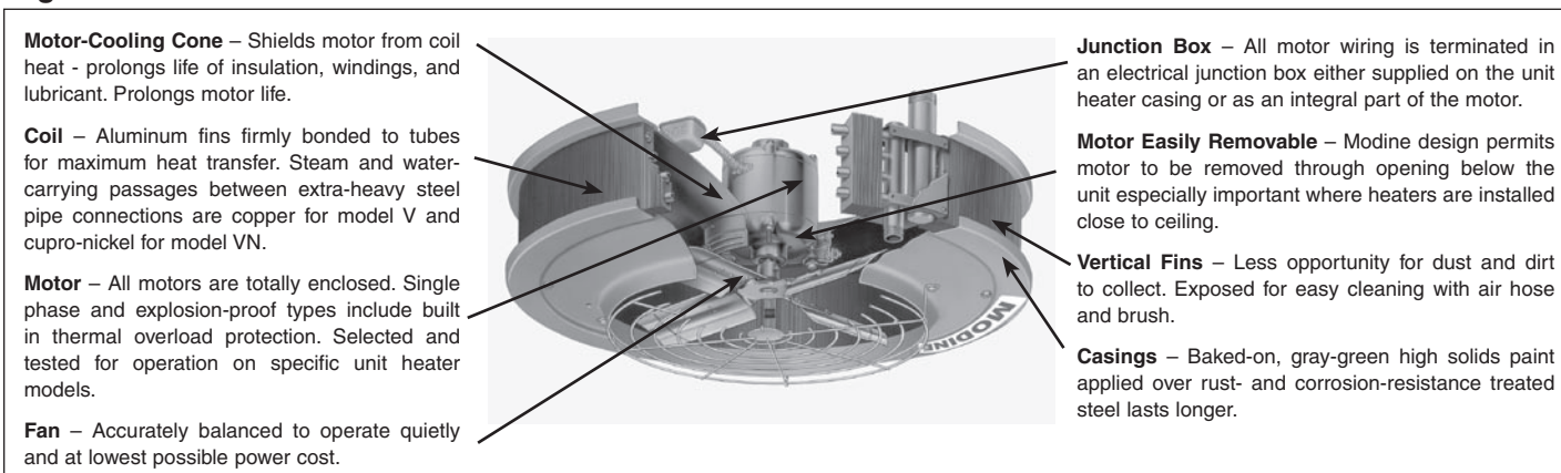
Figure 5.1 – Unit Features
