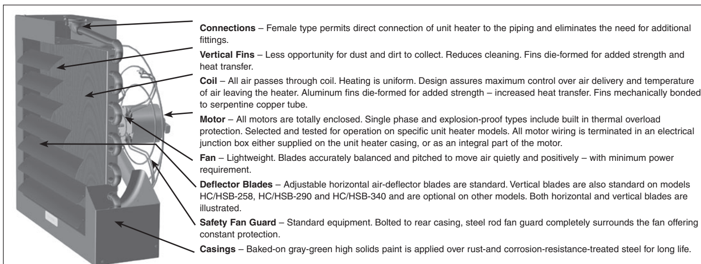
Figure 4.1 Unit Features
